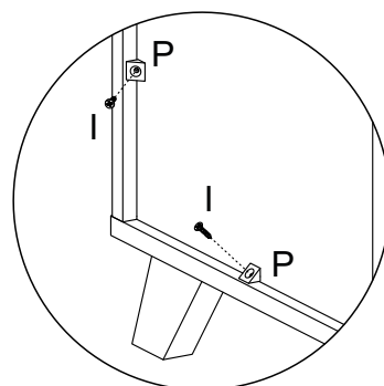
Detalhe 12 Detalle/Detail
