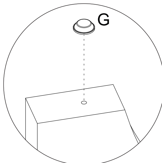
Detalhe 1 Detalle/Detail
