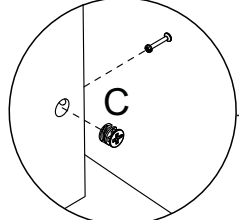
Detalhe 10 Detalle/Detail
