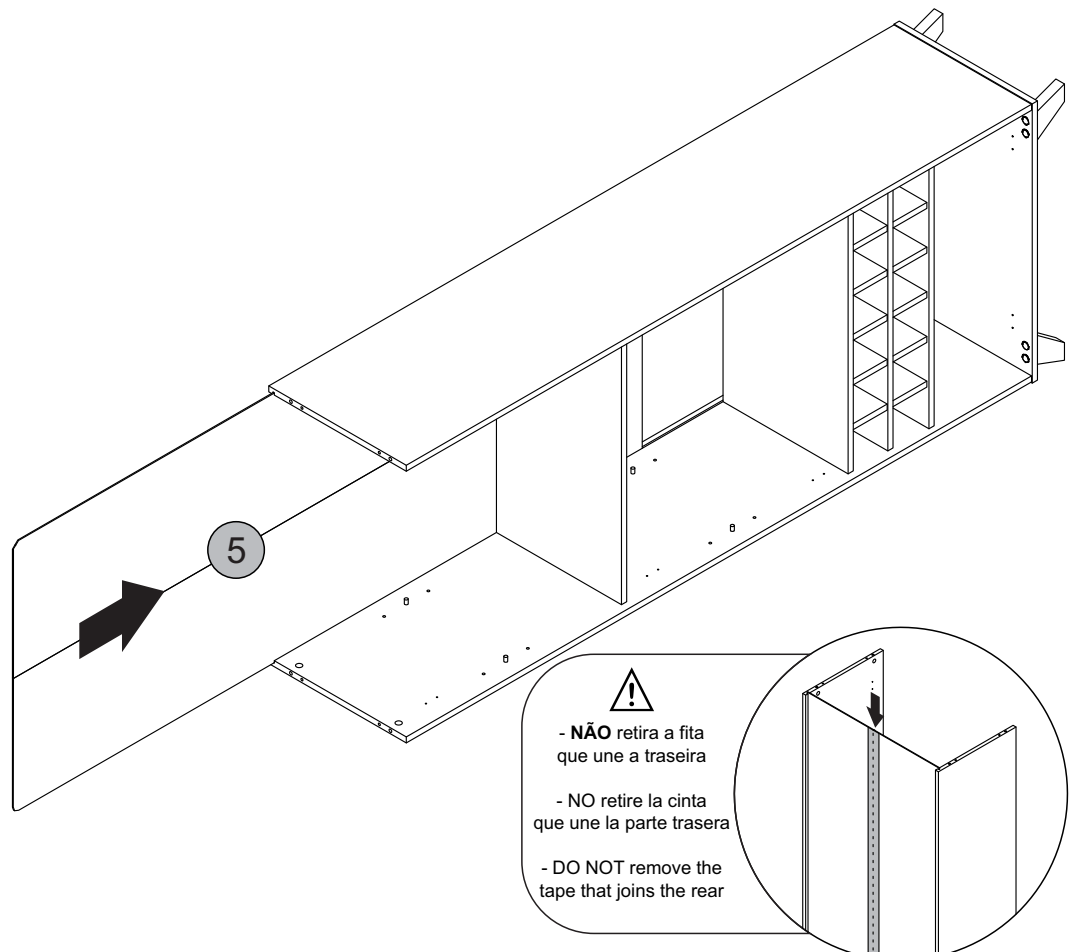
Detalhe 11 Detalle/Detail
