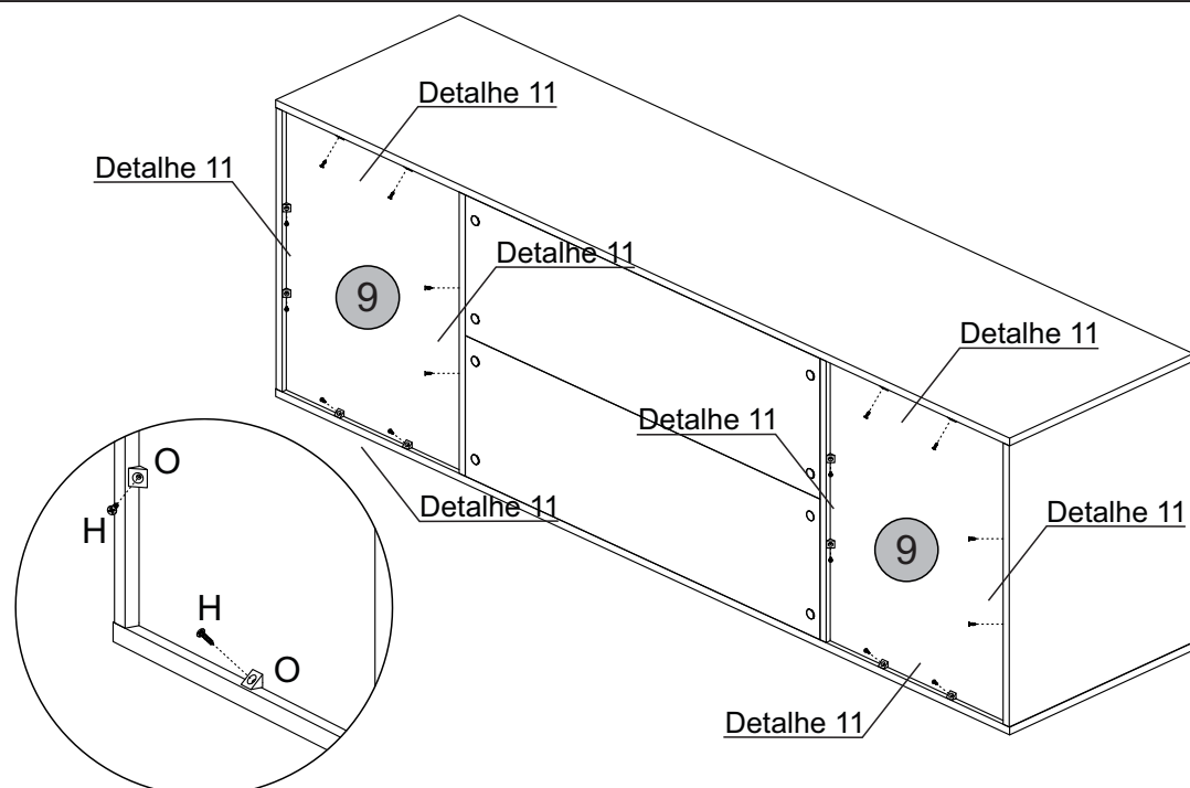
Detalhe 11 Detalle/Detail
