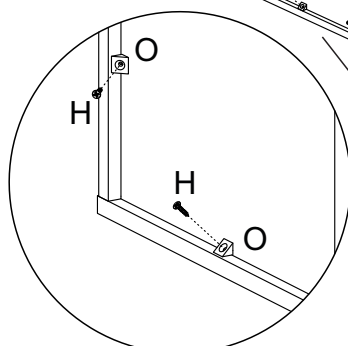
Detalhe 11 Detalle/Detail
