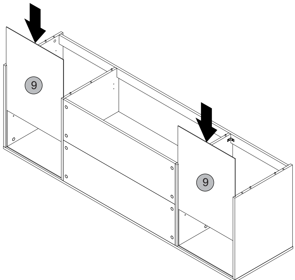
Detalhe 9 Detalle/Detail
